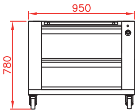
Heated base cabinet with drawers (Optional)
