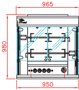
Front view Rotisserie with roof and base on casters (optional)
