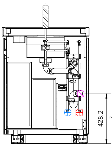
SECTION D
