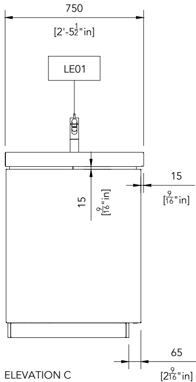
ELEVATION C
