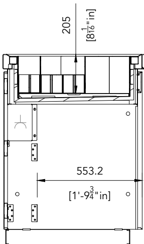
SECTION F
