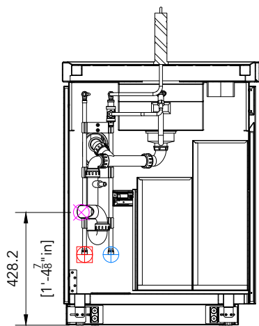
SECTION D
