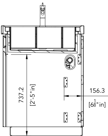
SECTION E
