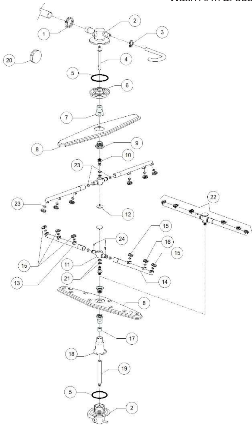
Wash Arm Group
