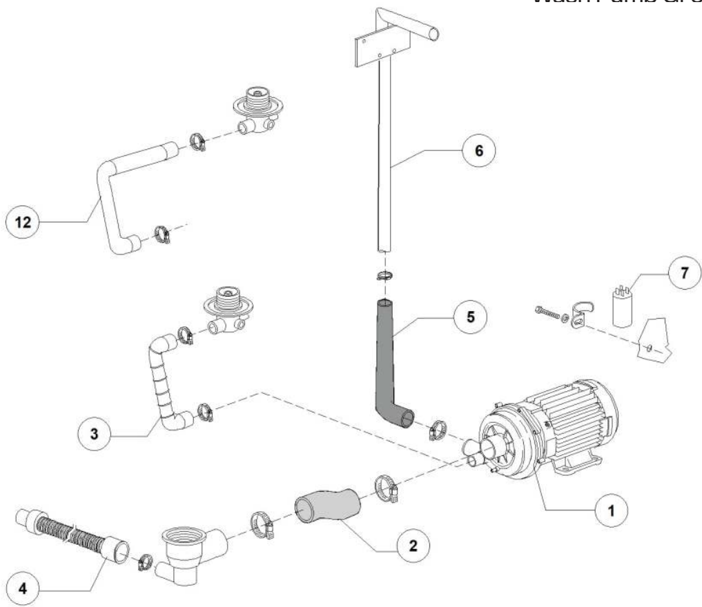
Wash Pump Group
