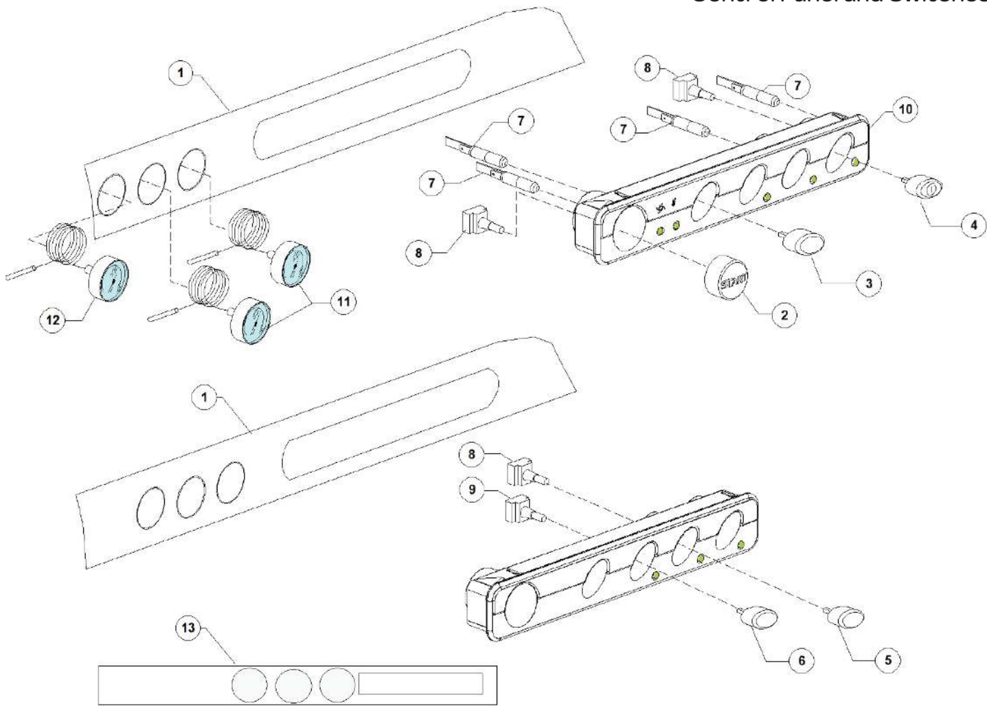
Control Panel and Switches
