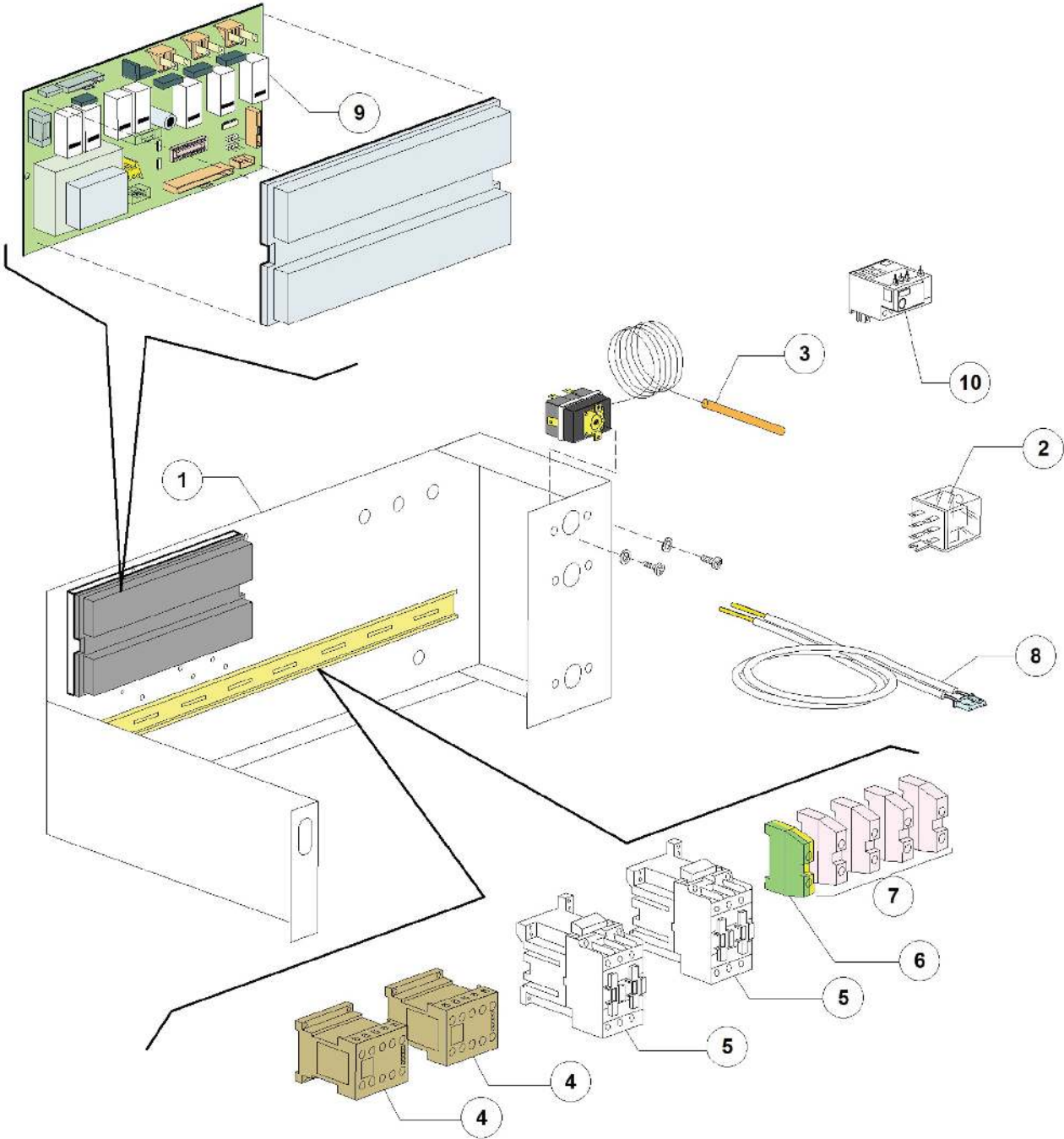
Electric Control Components
