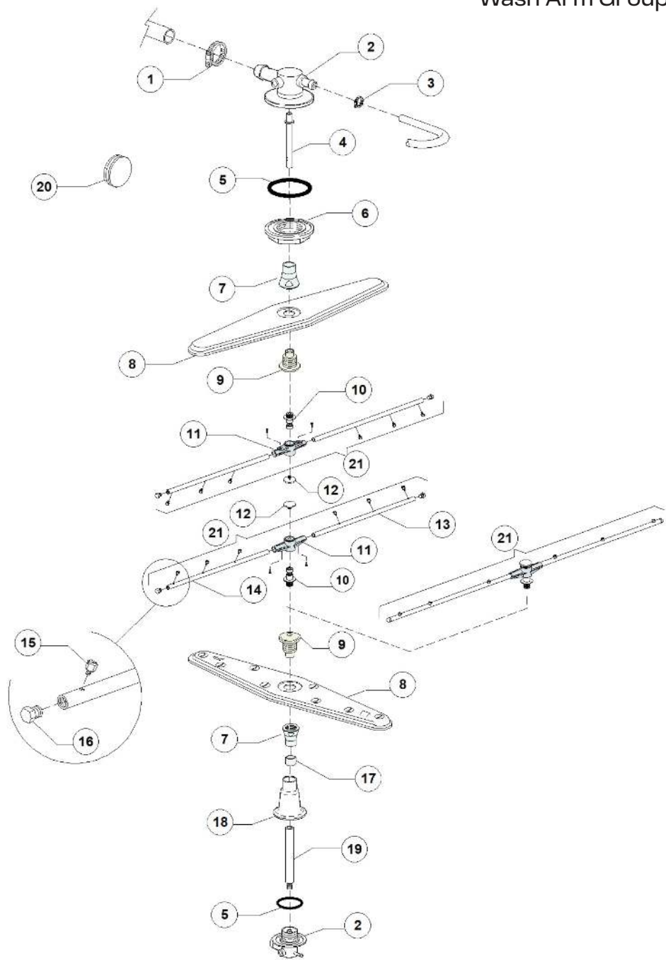
Wash Arm Group
