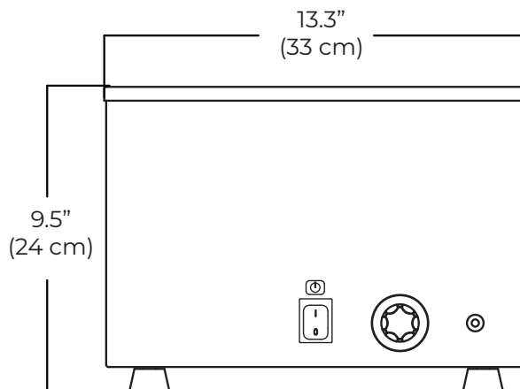
FRONTAL VIEW
