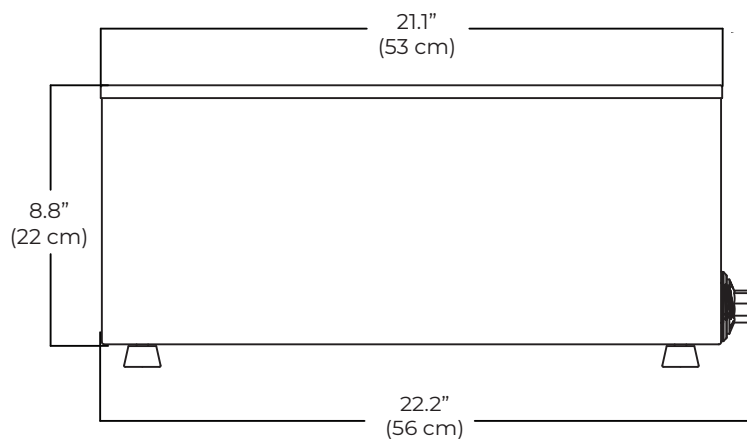
LEFT VIEW
