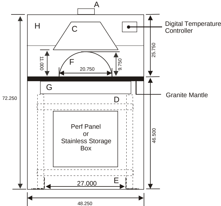
ELEVATION VIEW
