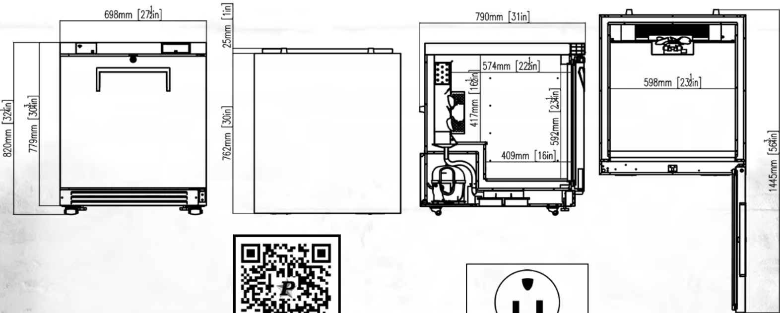
PRODUCT DRAWINGS
