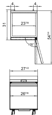
AWR27SD/AWF27SD
