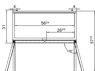
AWR60SD / AWF60SD
