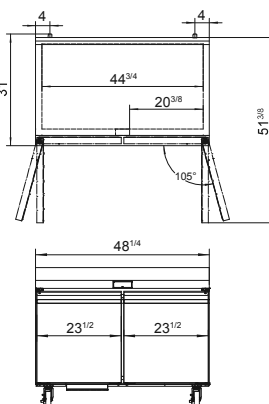
AWR48SD / AWF48SD
